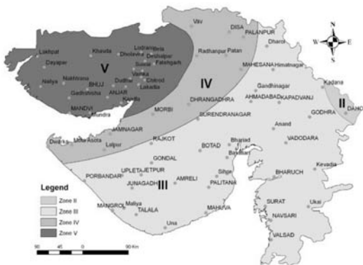
Figure 4: Seismicity Zoning Map - Gujarat, India
