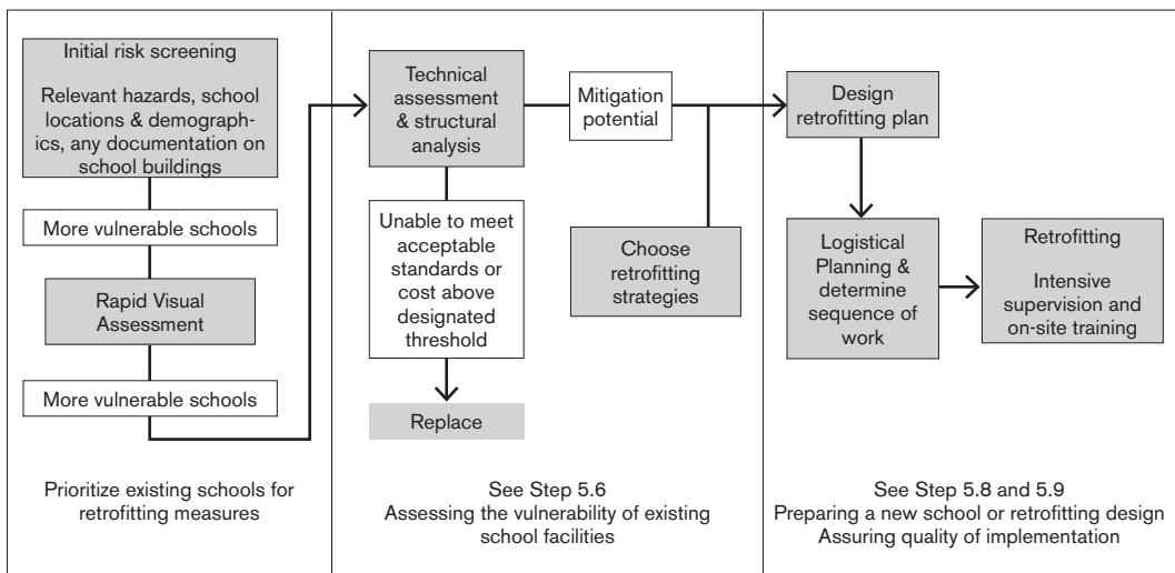
Figure 5: Example of Retrofit Workflow Diagram
