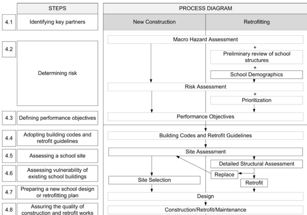
Figure 2: Safer School Steps and Corresponding Process Flow Diagram
